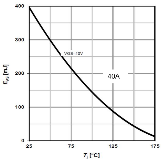
Avalanche energy
