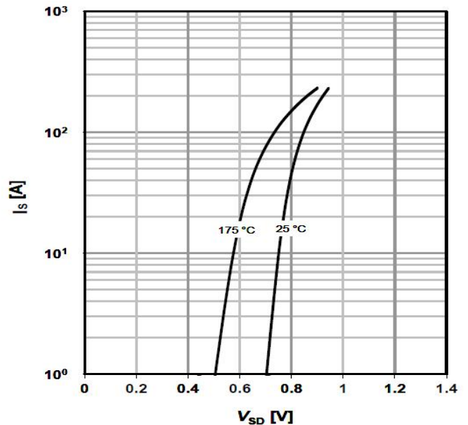
IS -- VSD
