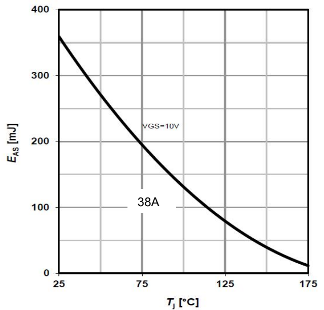
Avalanche energy
